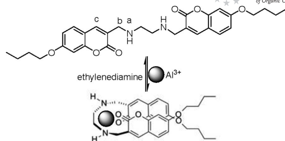
Figure 4. Proposed binding mode of 1 with \text{Al}^{3+} .
