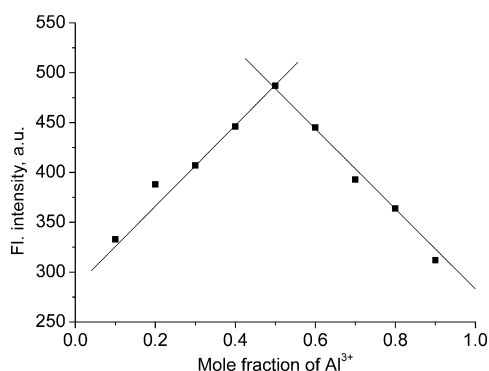
Figure 3. Job plot for the determination of the stoichiometry of sensor 1 and \text{Al}^{3+} . The total concentration of 1 and \text{Al}^{3+} was kept constant ( 25 \mu\text{M} ). Excitation and emission was at 340 and 395 nm, respectively.
